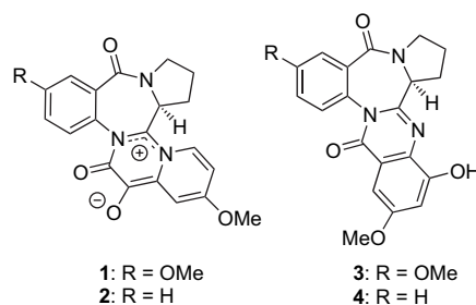
Scheme 1. The Circumdatins A, B, D, E.
