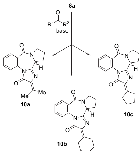
Scheme 3. Exploiting the CH-acidity of ring system 8a .
