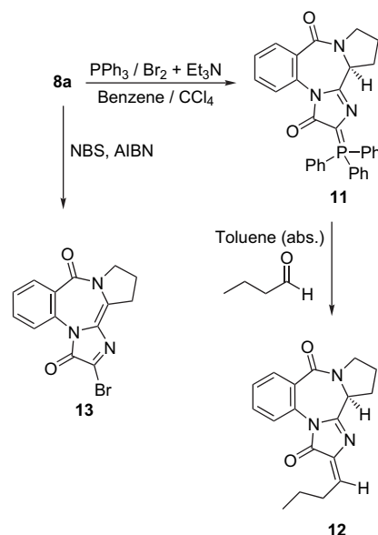
Scheme 4.
