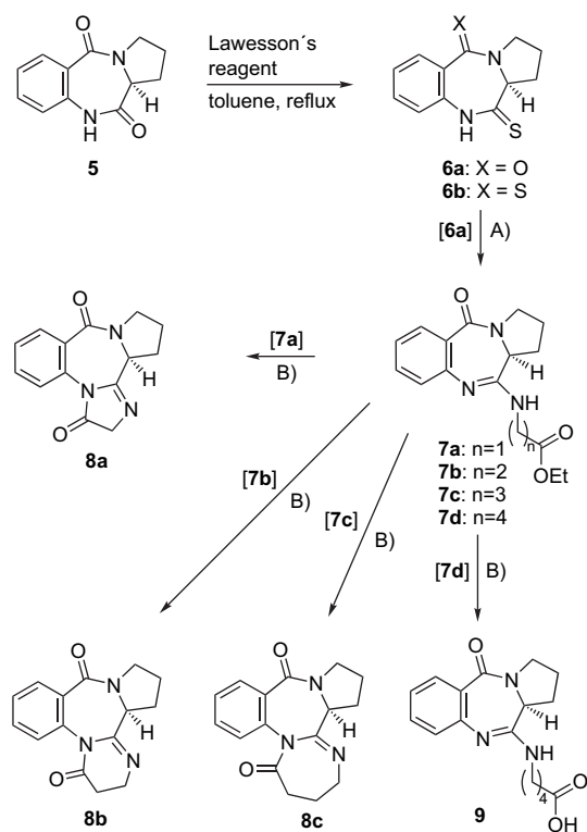
Scheme 2. Synthesis of new ring systems starting from monothiolactam 6a . Reaction conditions: (A) EtOOC-(CH 2 ) n -NH 3 + Cl - , HgCl 2 , NEt 3 ; (B) (1) NaOH, dioxane, H 2 O; (2) HCl.
