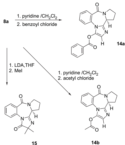
Scheme 5. Acylations and methylations of 8a .
